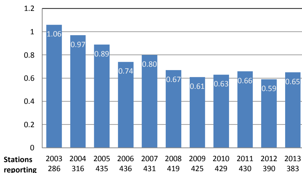
FIG. A-16. Mean rate of scrams: the number of automatic and manual scrams that occur per 7000 hours of operation. (Source: IAEA Power Reactor Information System http://www.iaea.org/pris )
