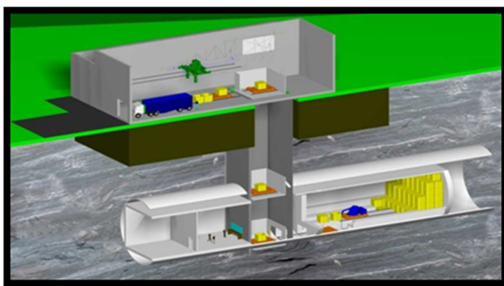
FIG. A-15. Concept of emplacement operations at the Russian Federation's planned LLW disposal facility. (Graphic: All-Russia Design and Research Institute for Integrated Power Technology)
