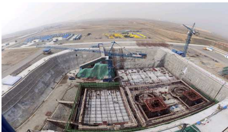
FIG. B-2. Construction site of the HTR-PM at Shidao Bay, Weihai City, China. (Photo: Institute of Nuclear and New Energy Technology)
