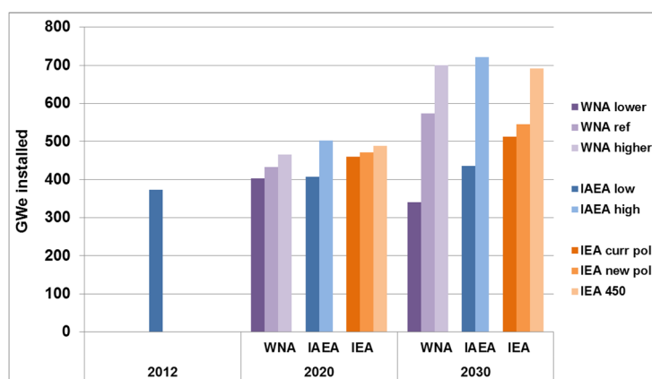
FIG. A-7. Comparison of nuclear power projections from the IAEA, the WNA and the IEA.
