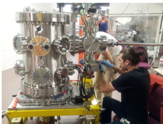
FIG. C-2: Assembly of the UHVC end-station.
