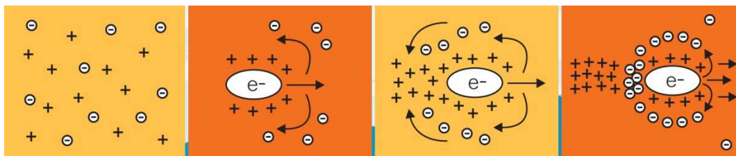
FIG. C-1. From left: (a) Positive ions and free electrons forming a plasma, (b) An electron bunch enters the plasma and repels all free electrons. Positive ions are attracted around the bunch, (c) The already displaced free electrons are now attracted by the positive ions left behind the bunch, (d) The free electrons in their new position behind the bunch give the electron bunch an acceleration.
