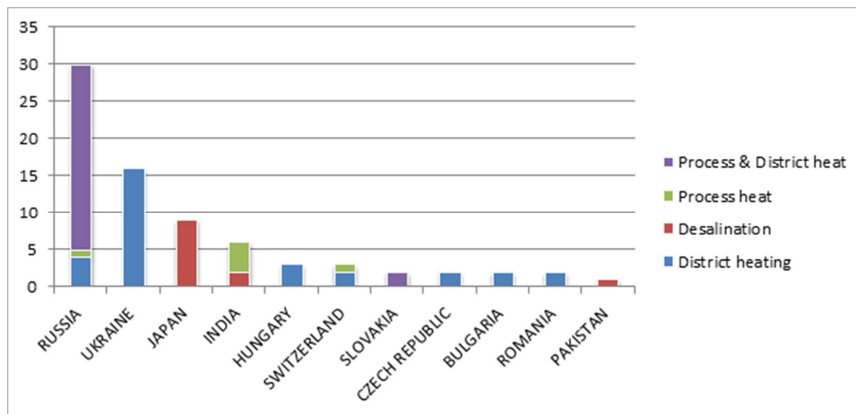
FIG. A-6. Number of reactors used for both non-electric purposes and for electricity production.
