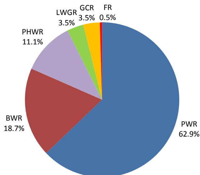
FIG. A-1. Current distribution of reactor types. (BWR: boiling water reactor; FR: fast reactor; GCR: gas cooled reactor; LWGR: light water cooled, graphite moderated reactor; PHWR: pressurized heavy water reactor; PWR: pressurized water reactor).
