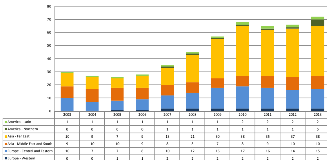
FIG. A-3. Number of reactors under construction by region
