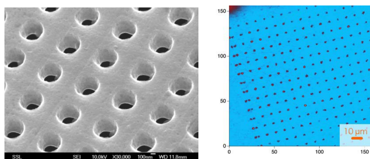
FIG. C-2. Left: Scanning electron microscope image of a uniform array of holes with diameters of a few hundred nanometres in silicon. (Photo: M.B.H. Breese/National University of Singapore). Right: Confocal microscope image of lattice of nitrogen–vacancy centres created by ion implantation of diamond. A few nitrogen-15 ions were irradiated into each irradiation spot. (Photo: T. Ohshima/Japan Atomic Energy Commission).
