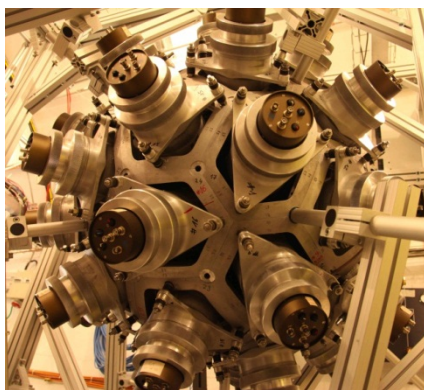
FIG. B-1. Detectors at the n_TOF facility at CERN. (Photo: CERN)
