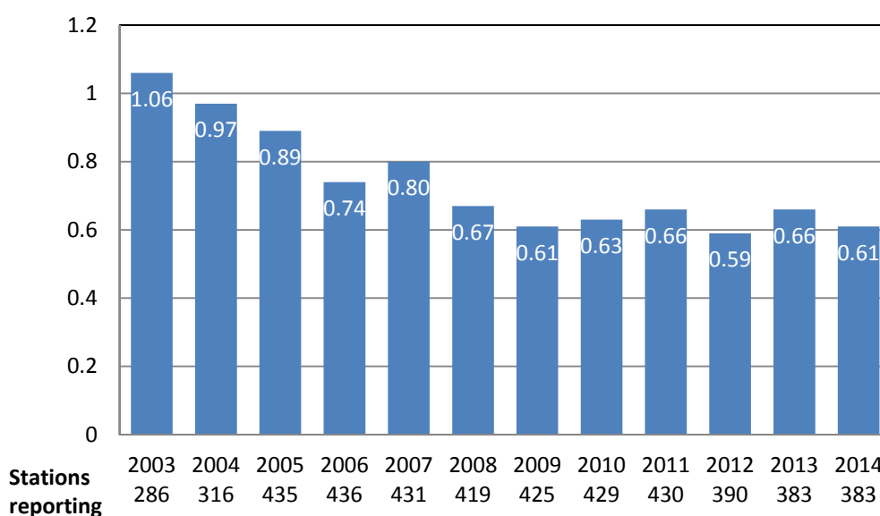
FIG. A-13. Mean rate of scrams: the average, annual number of automatic and manual scrams. (Source: The Agency's Power Reactor Information System http://www.iaea.org/pris )
