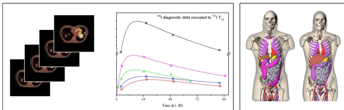
FIG. E-2. Left: Series of images and derived time-activity curves for different source organs. Right: an example of mathematical phantoms used for S value calculations.
