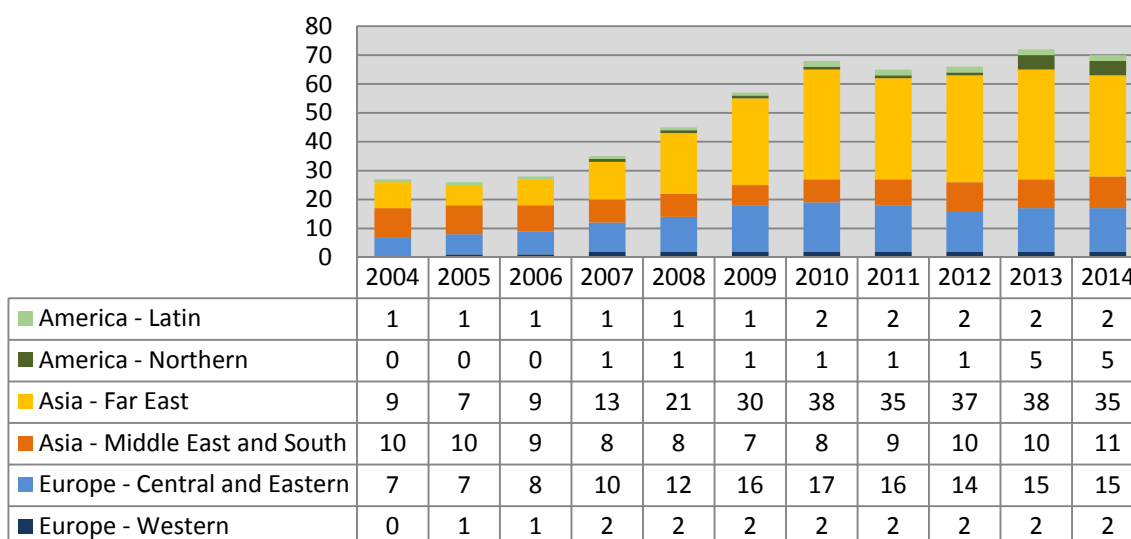
FIG. A-2. Number of reactors under construction by region.
