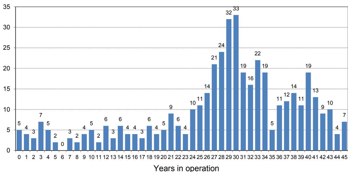
FIG. A-3. Distribution of operational power reactors by age as of 31 December 2014. (Source: The Agency's Power Reactor Information System http://www.iaea.org/pris )
